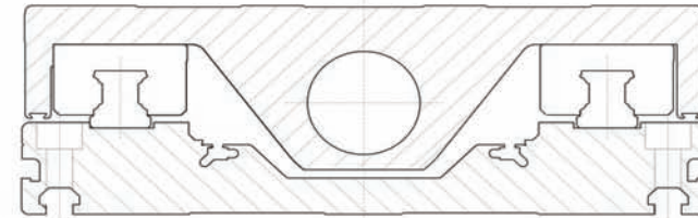
TT225 with ball bearing guides Outer dimensions: 225x75
