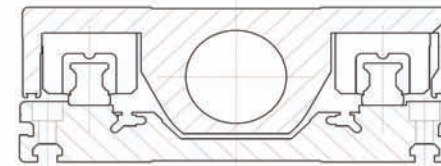
TT155 with ball bearing guides Outer dimensions: 155x60
