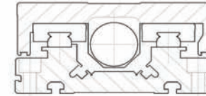
TT100 with ball bearing guides Outer dimensions: 100x50
